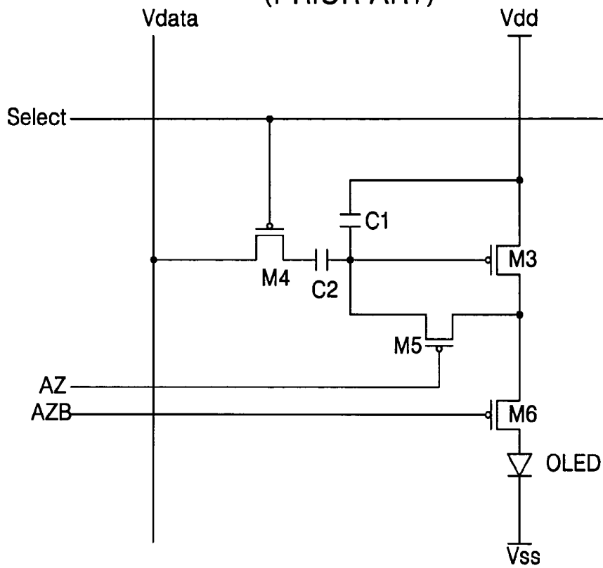
FIG. 3 (PRIOR ART)
